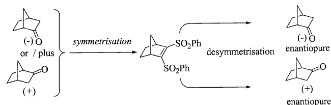
Figure 4. Total resolution of norcamphor
