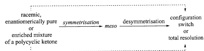
Figure 3. Double role of “symmetrisation”/“desymmetrisation” strategy
